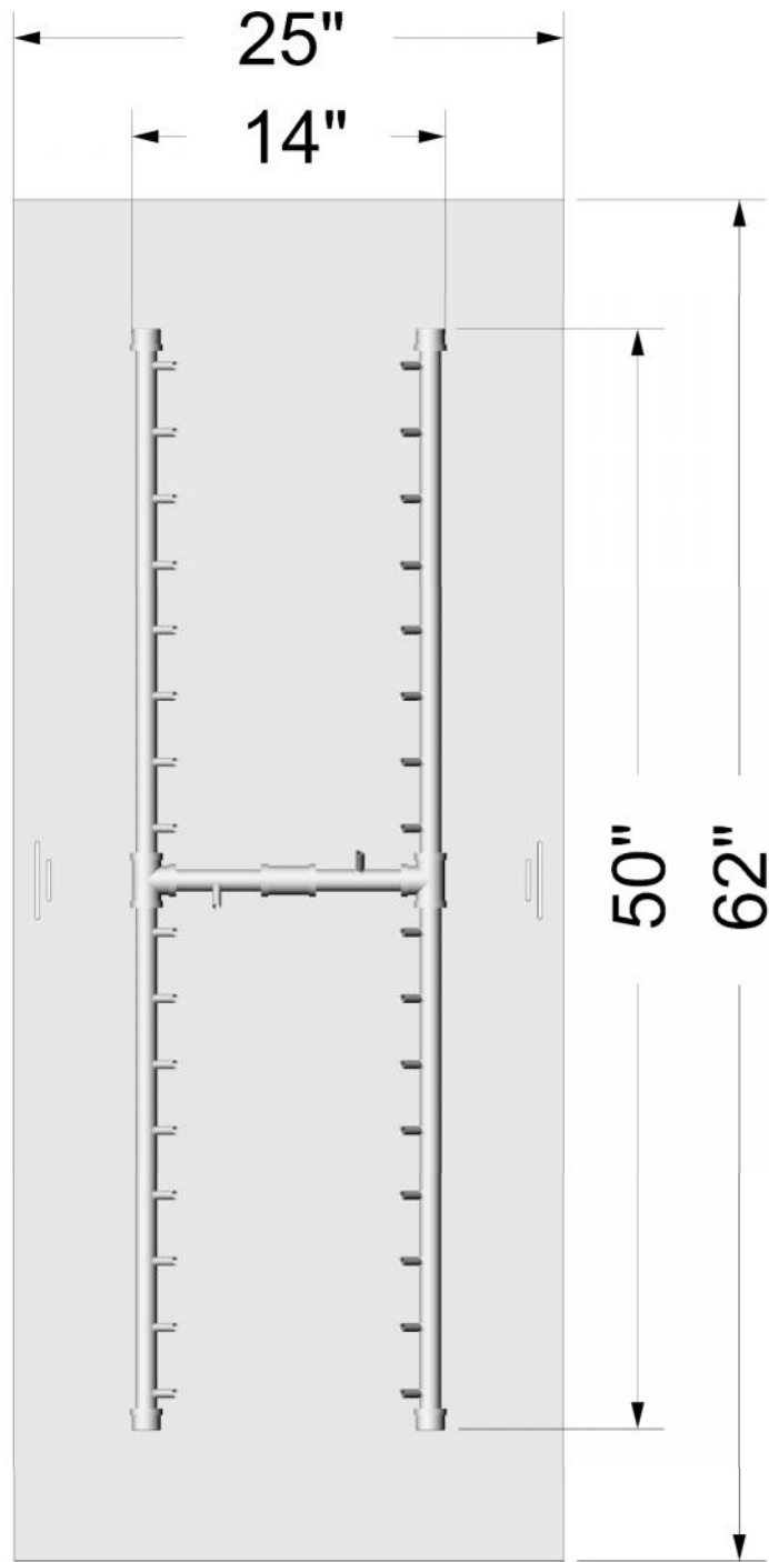
Rectangular Plate: Top View
