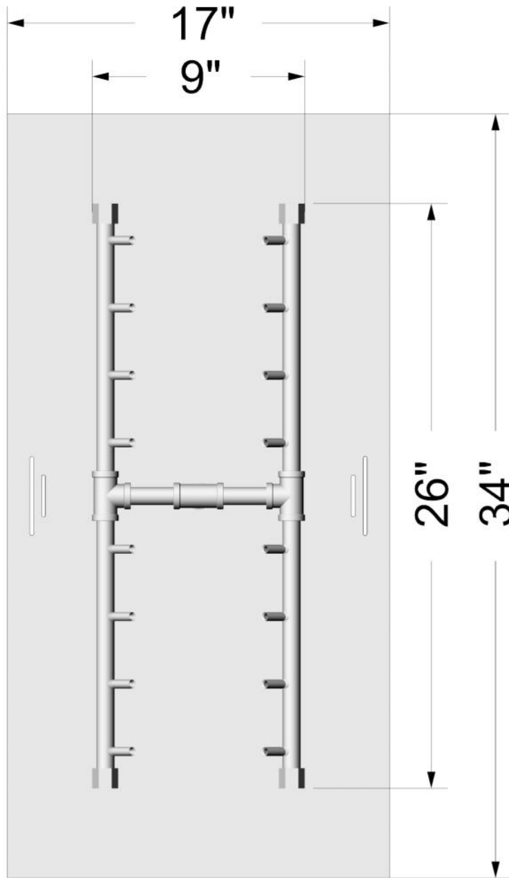
Rectangular Plate: Top View
